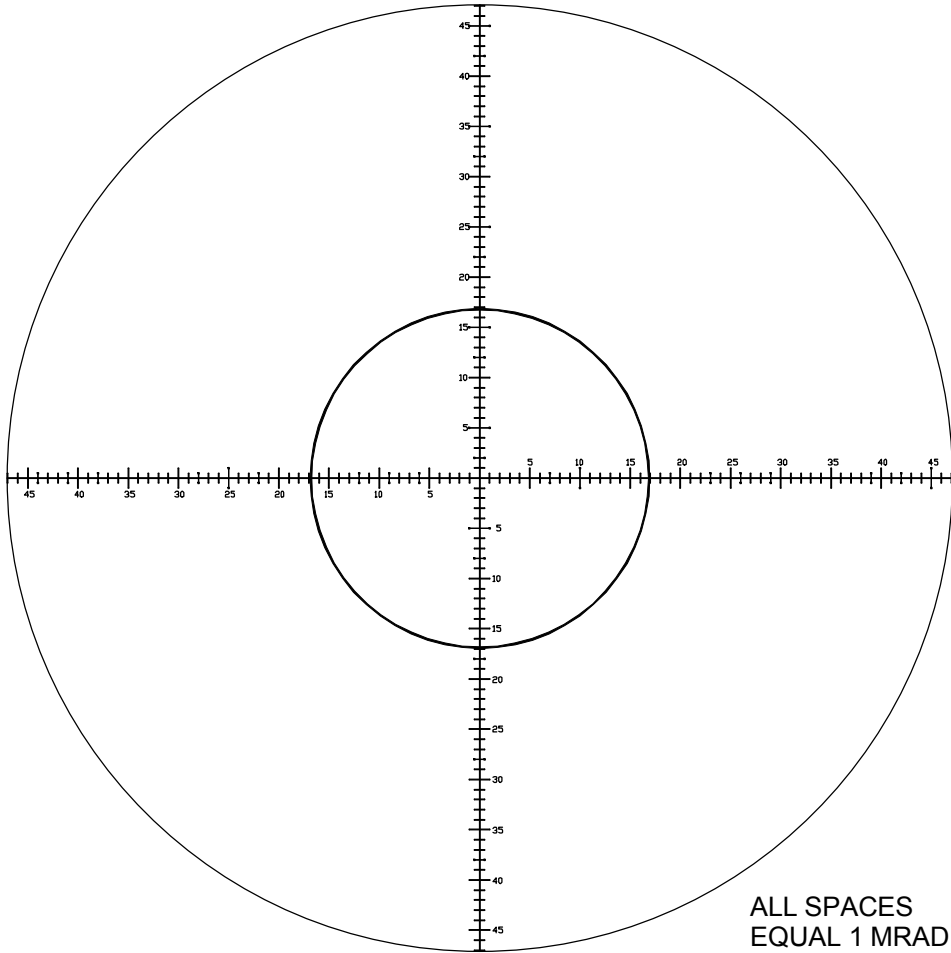
Graduated Reticle (Example)
